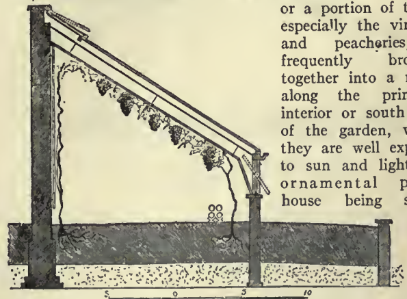
FIG. 5.—Lean-to Vinery.
